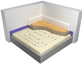
Spiral pipe layout (for rectangular shaped rooms where even spread of heat is required)
