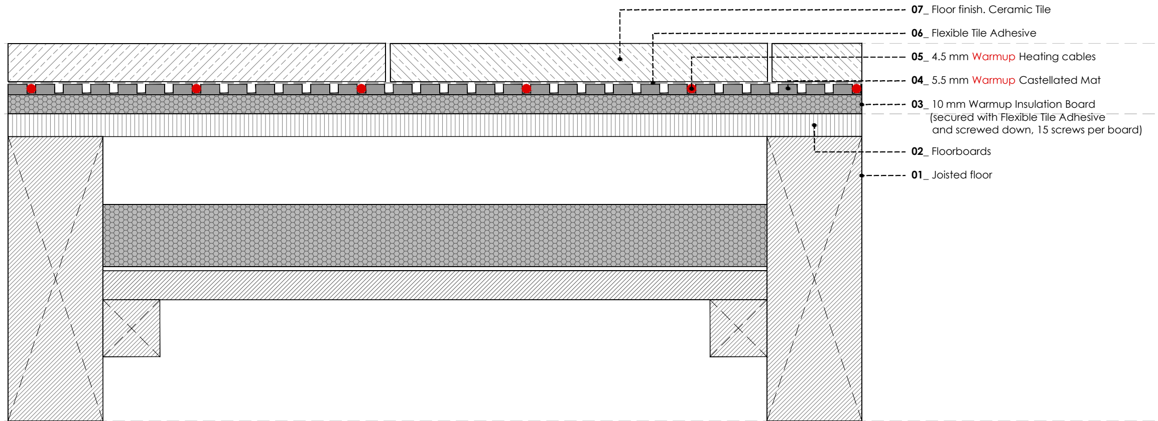
WARMUP CASTELLATED MAT SYSTEM. TIMBER SUBFLOOR AND TILES (with Warmup insulation boards)
