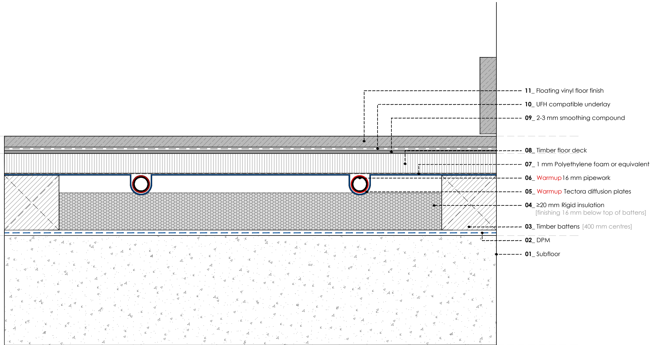
WARMUP TECTORA JOISTED BATTEN FLOOR SYSTEM. Concrete subfloor. Vinyl floor - floating
