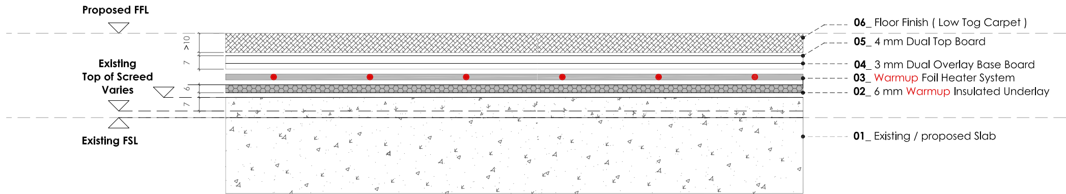
WARMUP UNDERFLOOR HEATING FOIL HEATER SYSTEM ( LOW TOG CARPET)
