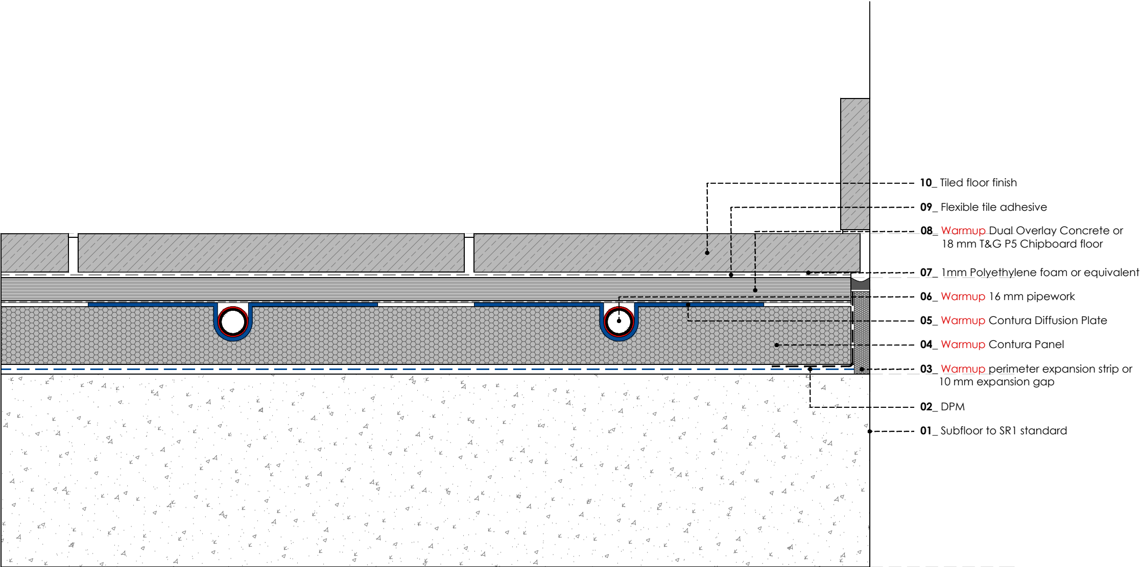
WARMUP CONTURA FLOATING FLOOR SYSTEM. Concrete subfloor. Tiled floor
