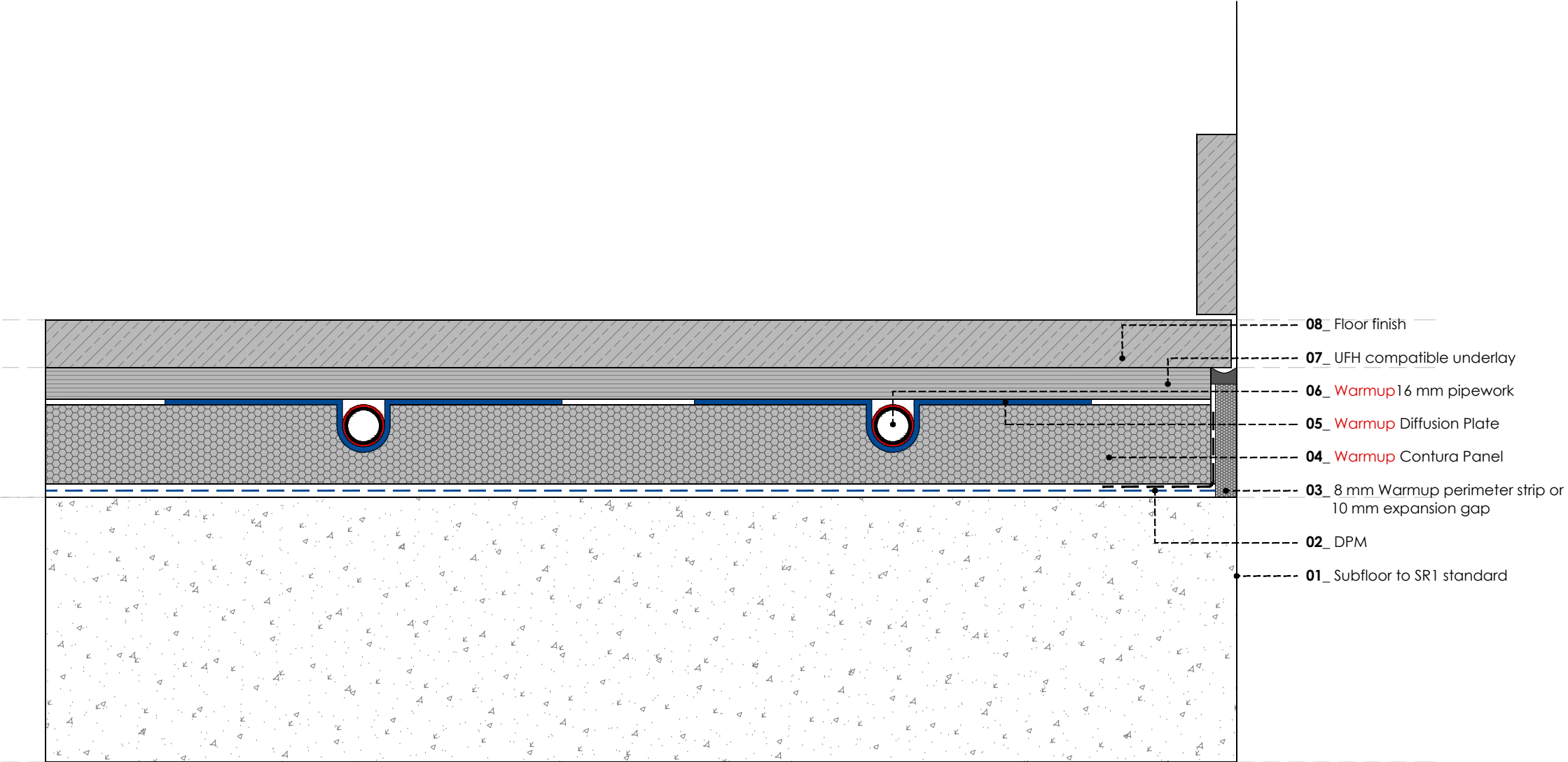
WARMUP CONTURA FLOATING FLOOR SYSTEM. Concrete subfloor. Generic template
