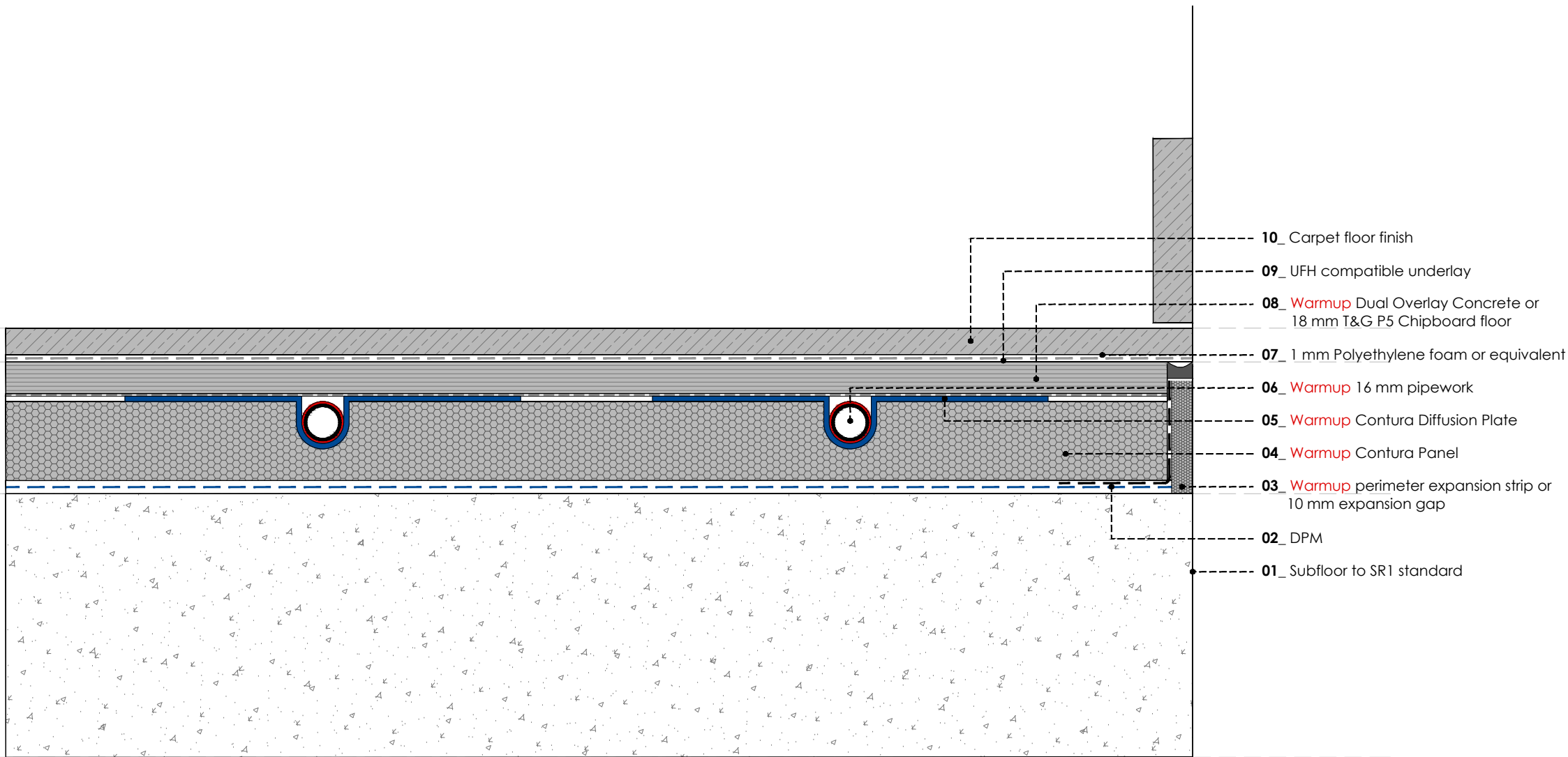
WARMUP CONTURA FLOATING FLOOR SYSTEM. Concrete subfloor. Carpet floor
