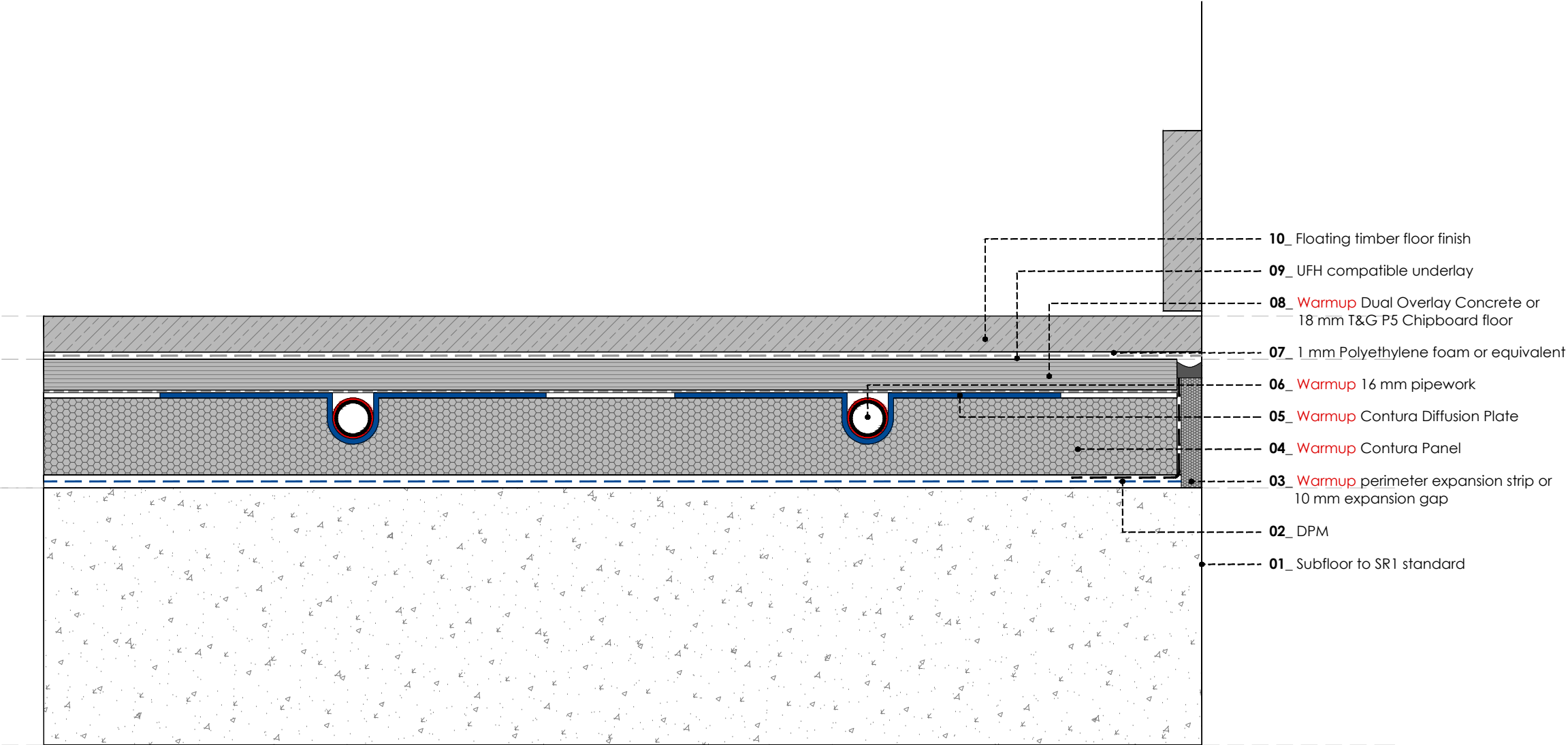
WARMUP CONTURA FLOATING FLOOR SYSTEM. Concrete subfloor. Wood / Laminate floor less than 14 mm - Floating
