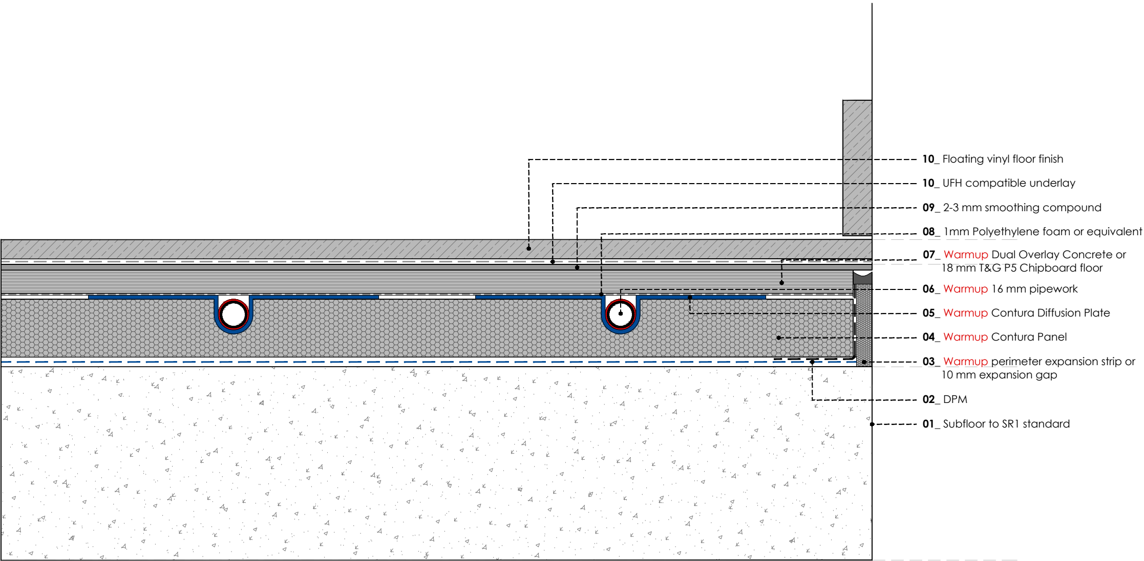
WARMUP CONTURA FLOATING FLOOR SYSTEM. Concrete subfloor.Vinyl floor - floating
