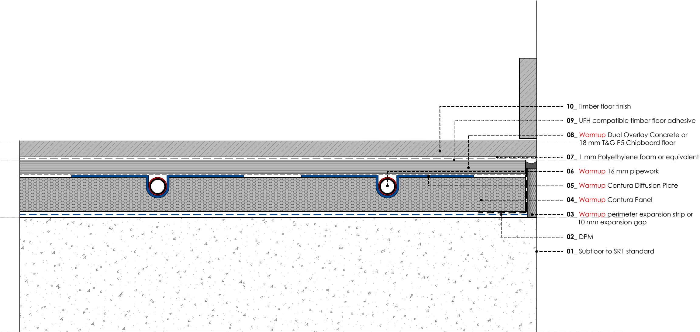
WARMUP CONTURA FLOATING FLOOR SYSTEM. Concrete subfloor. Wood / Laminate floor - glued
