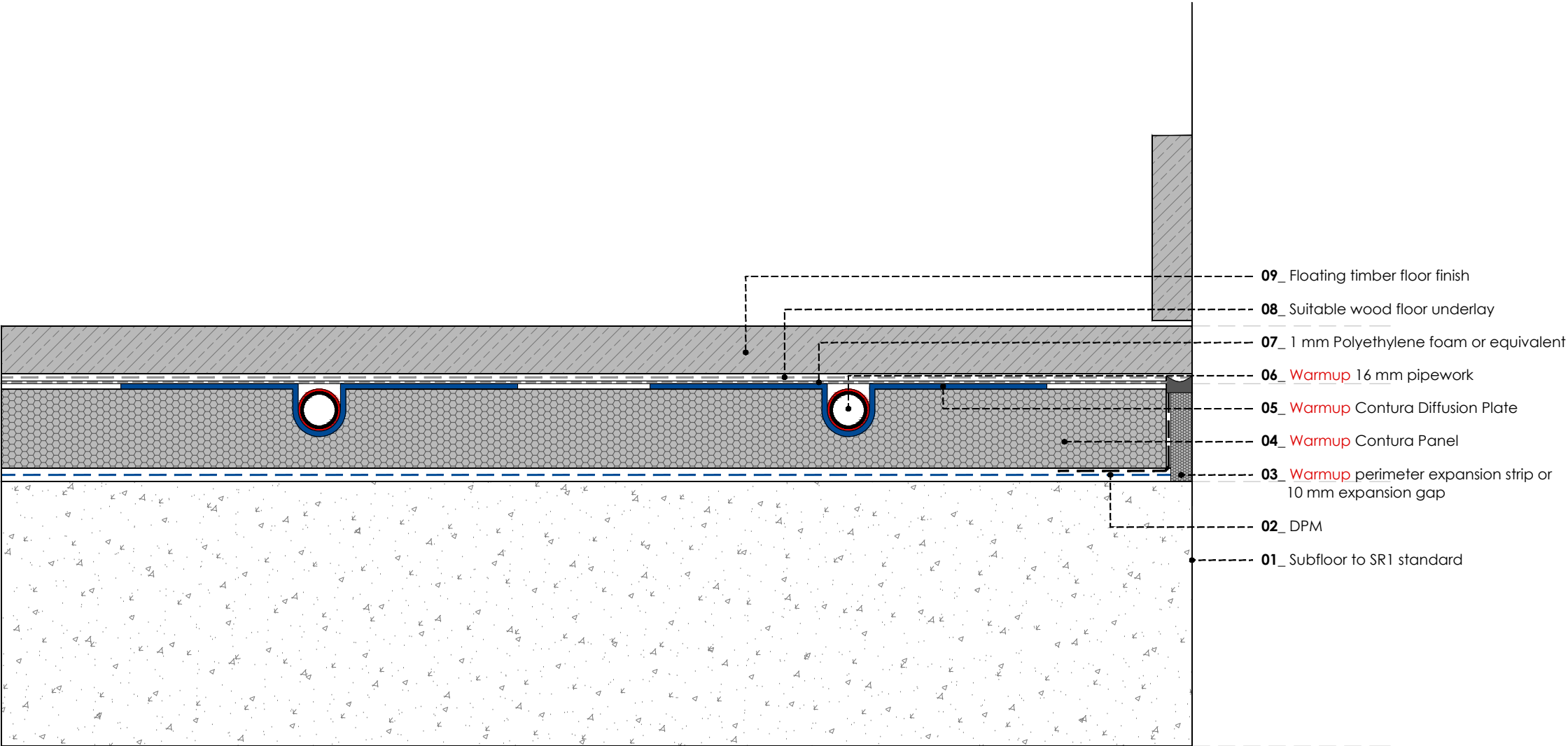
WARMUP CONTURA FLOATING FLOOR SYSTEM. Concrete subfloor. 14-25 mm Wood / Laminate floor - floating
