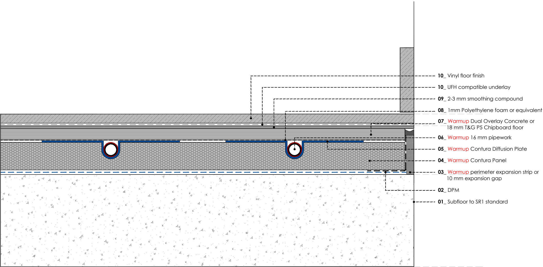
WARMUP CONTURA FLOATING FLOOR SYSTEM. Concrete subfloor. Vinyl floor - glued
