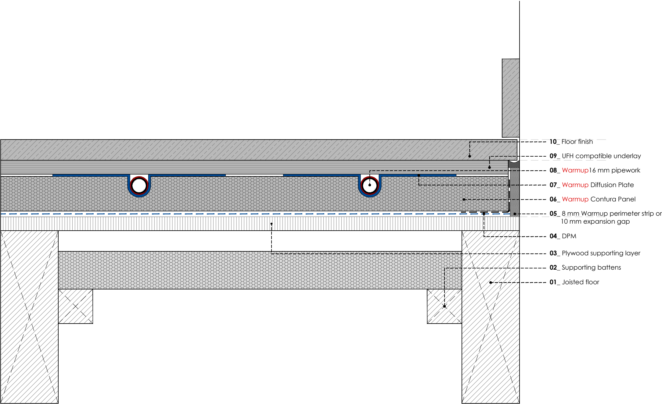
WARMUP CONTURA FLOATING FLOOR SYSTEM. Timber subfloor. Generic template
