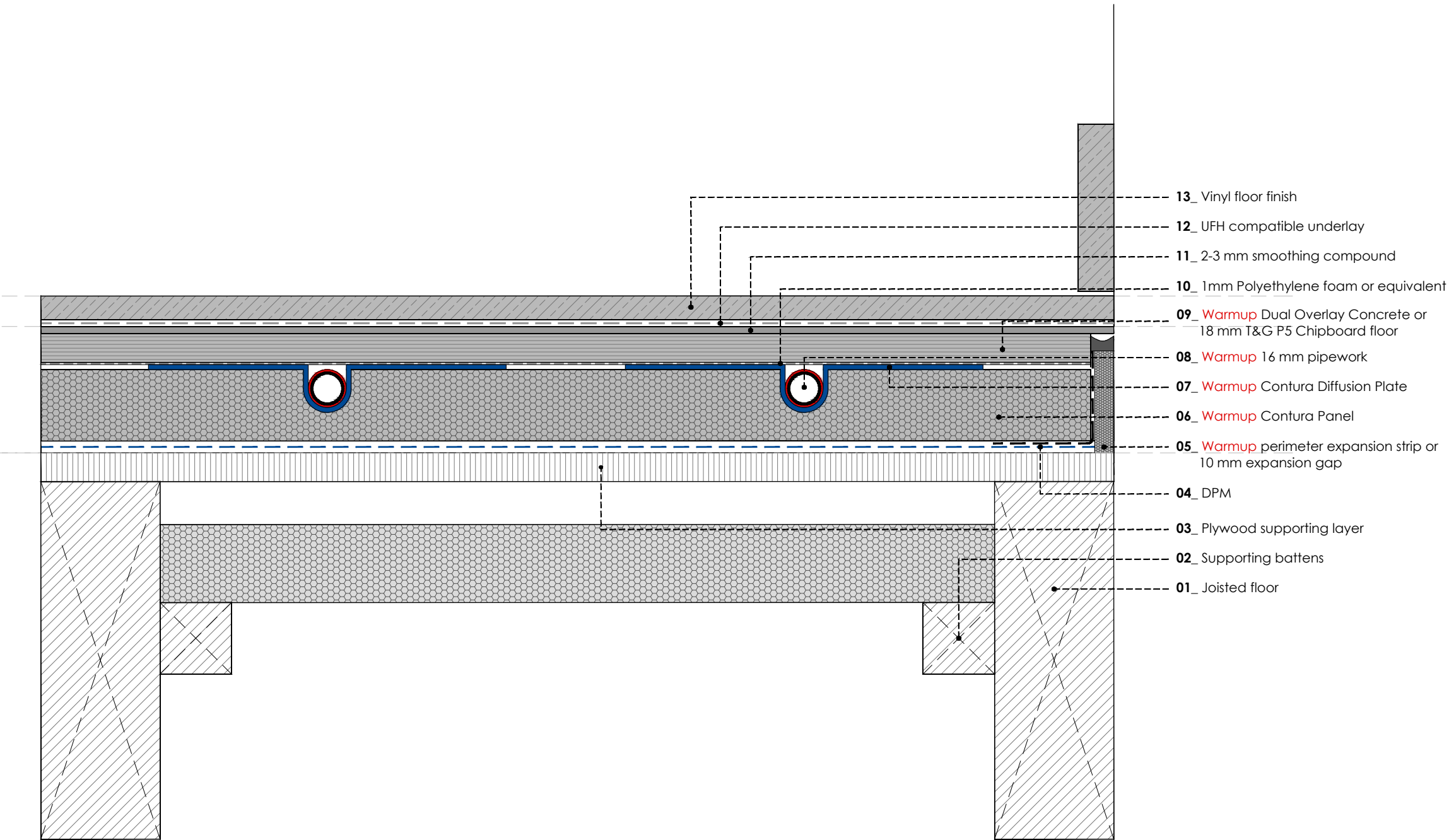
WARMUP CONTURA FLOATING FLOOR SYSTEM. Timber subfloor. Vinyl floor - glued
