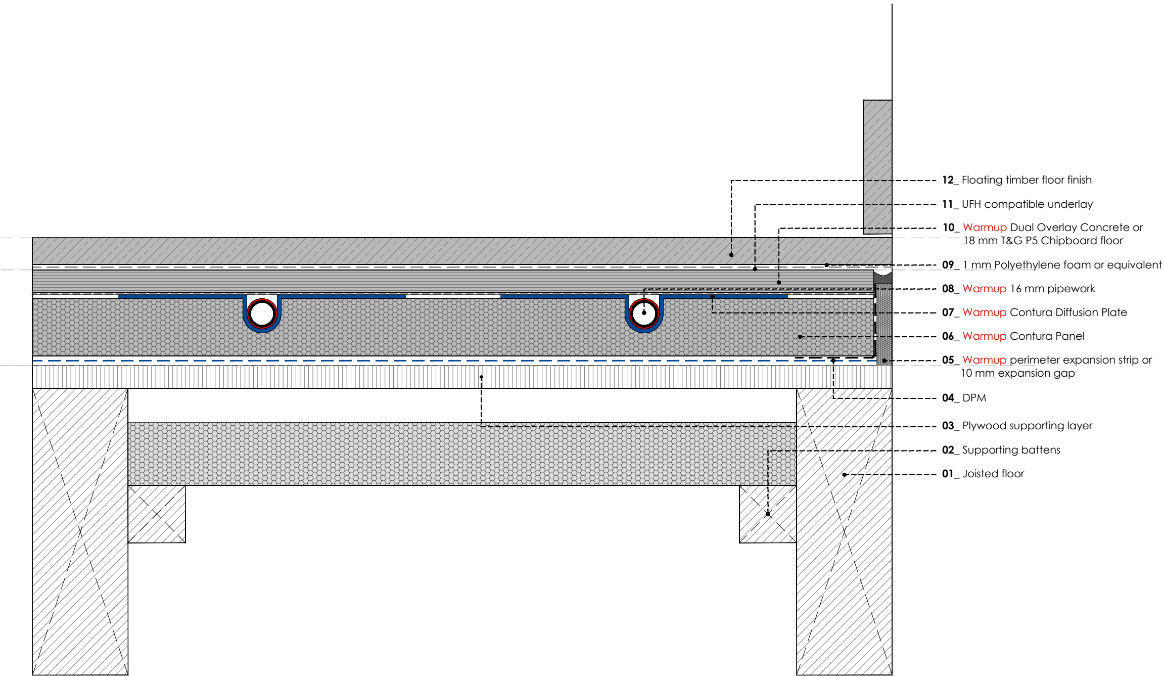
WARMUP CONTURA FLOATING FLOOR SYSTEM. Timber subfloor. Wood / Laminate floor less than 14 mm - Floating
