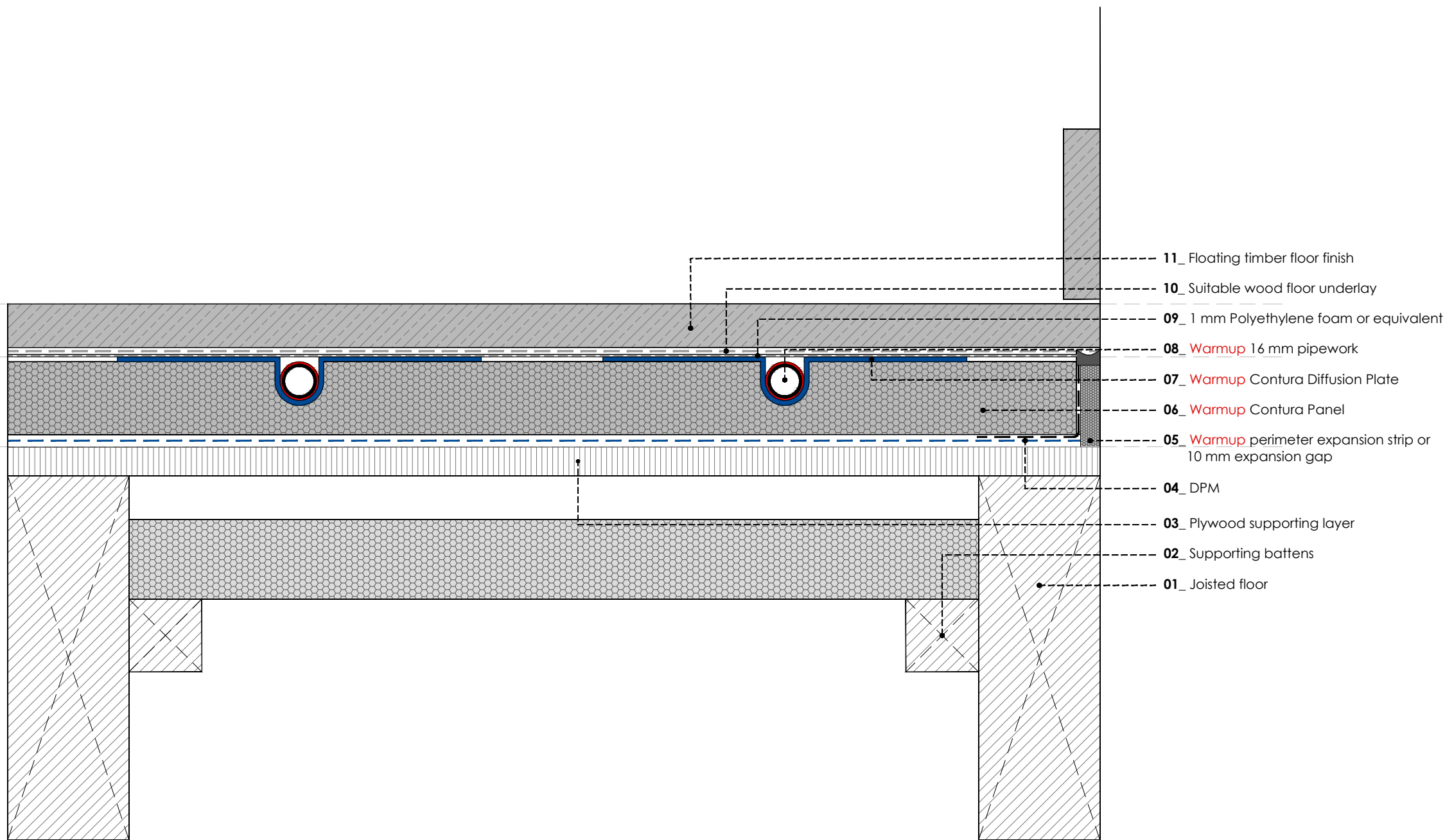
WARMUP CONTURA FLOATING FLOOR SYSTEM. Timber subfloor. Wood / Laminate floor - floating
