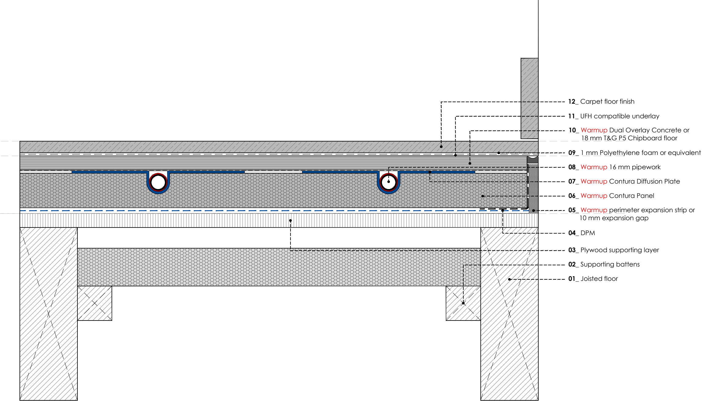
WARMUP CONTURA FLOATING FLOOR SYSTEM. Timber subfloor. Carpet floor
