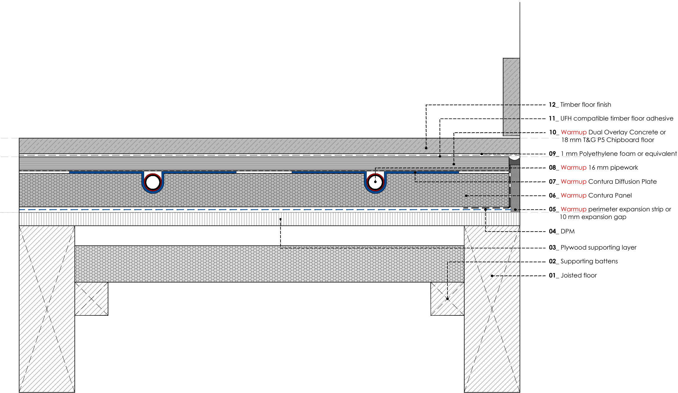
WARMUP CONTURA FLOATING FLOOR SYSTEM. Timber subfloor. Wood / Laminate floor - glued
