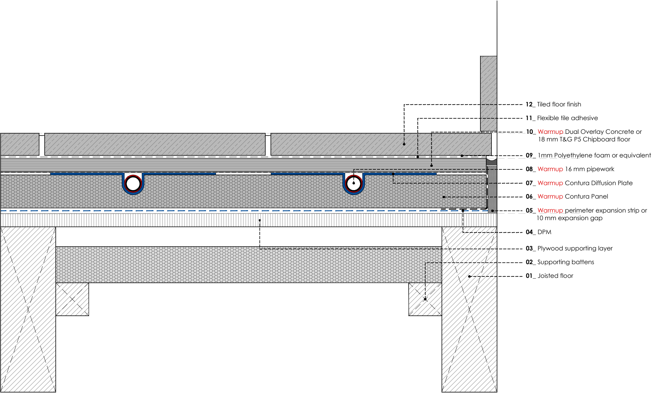
WARMUP CONTURA FLOATING FLOOR SYSTEM. Timber subfloor. Tiled floor
