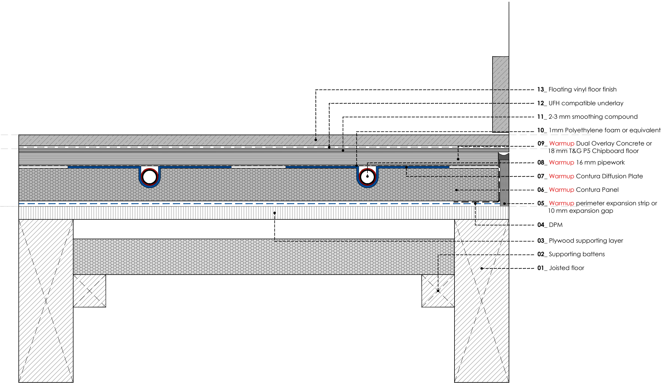
WARMUP CONTURA FLOATING FLOOR SYSTEM. Timber subfloor.Vinyl floor - floating
