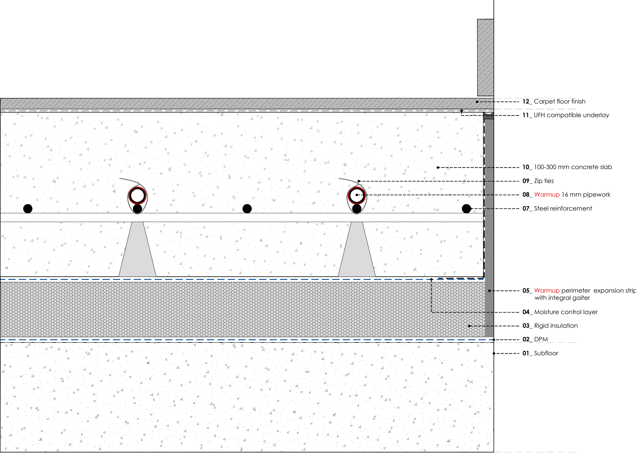
WARMUP FORTE GRID SYSTEM. Vinyl floor - glued
