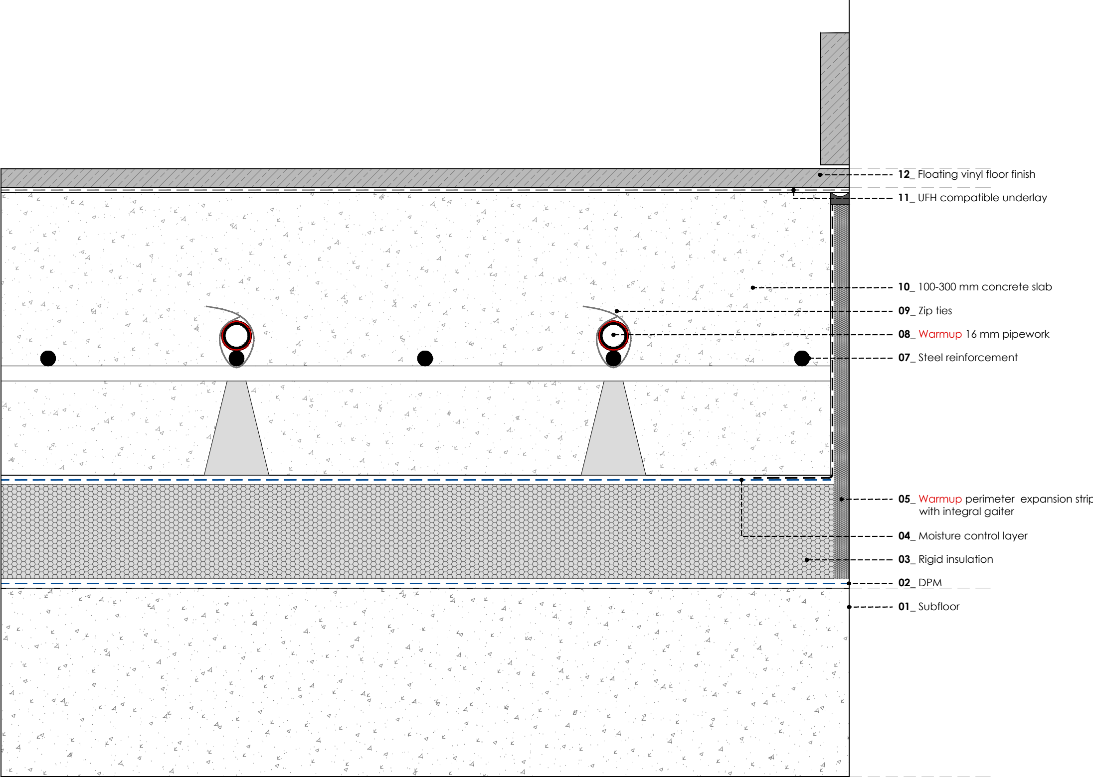
WARMUP FORTE GRID SYSTEM. Vinyl floor - floating
