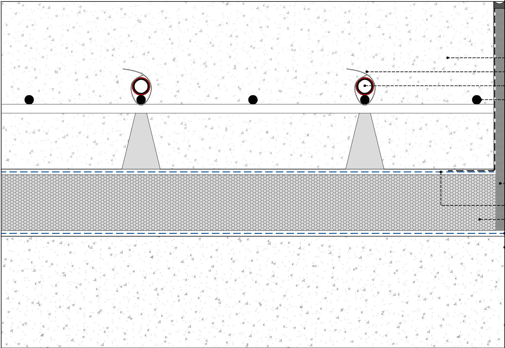
WARMUP FORTE GRID SYSTEM. Concrete floor
