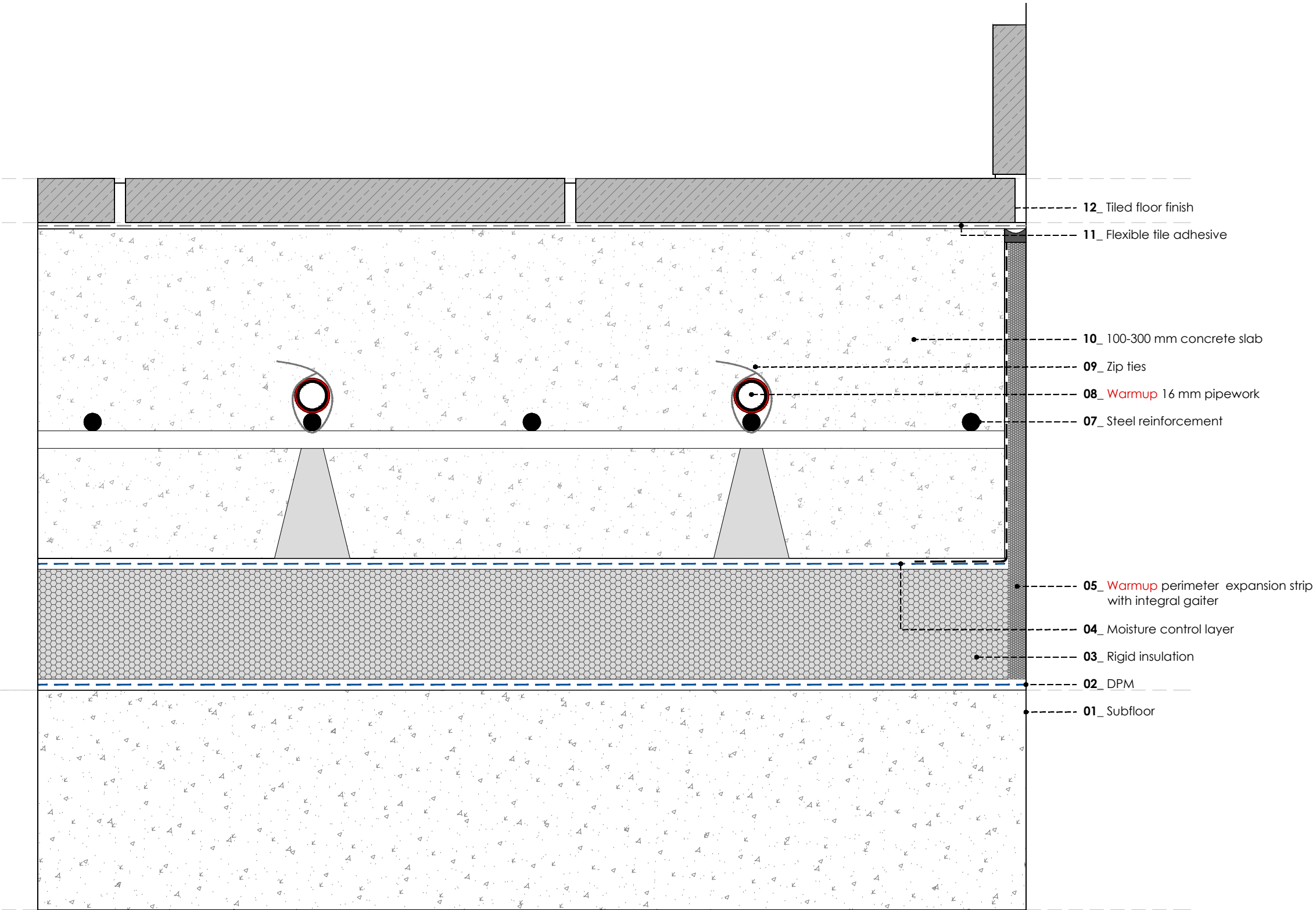
WARMUP FORTE GRID SYSTEM. Tiled floor
