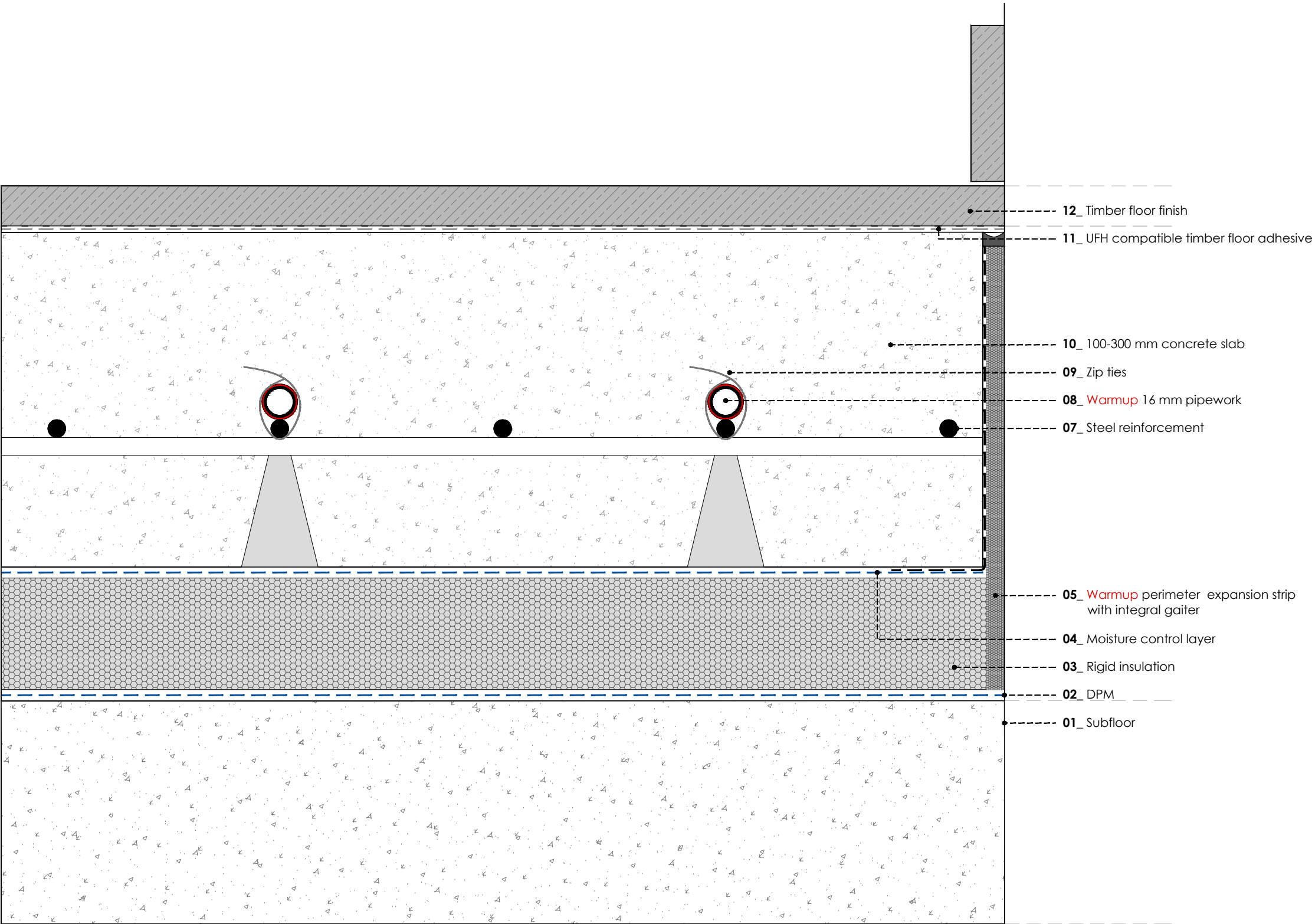
WARMUP FORTE GRID SYSTEM. Wood / Laminate floor - glued
