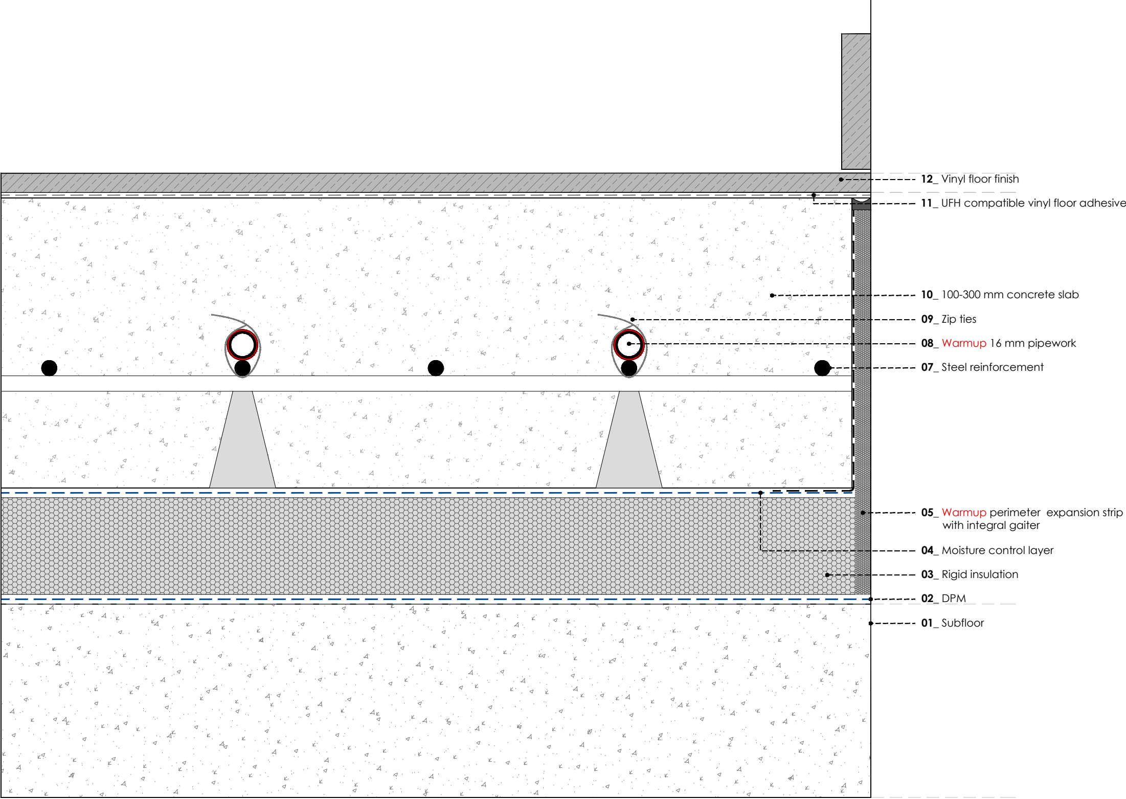
WARMUP FORTE GRID SYSTEM. Vinyl floor - glued
