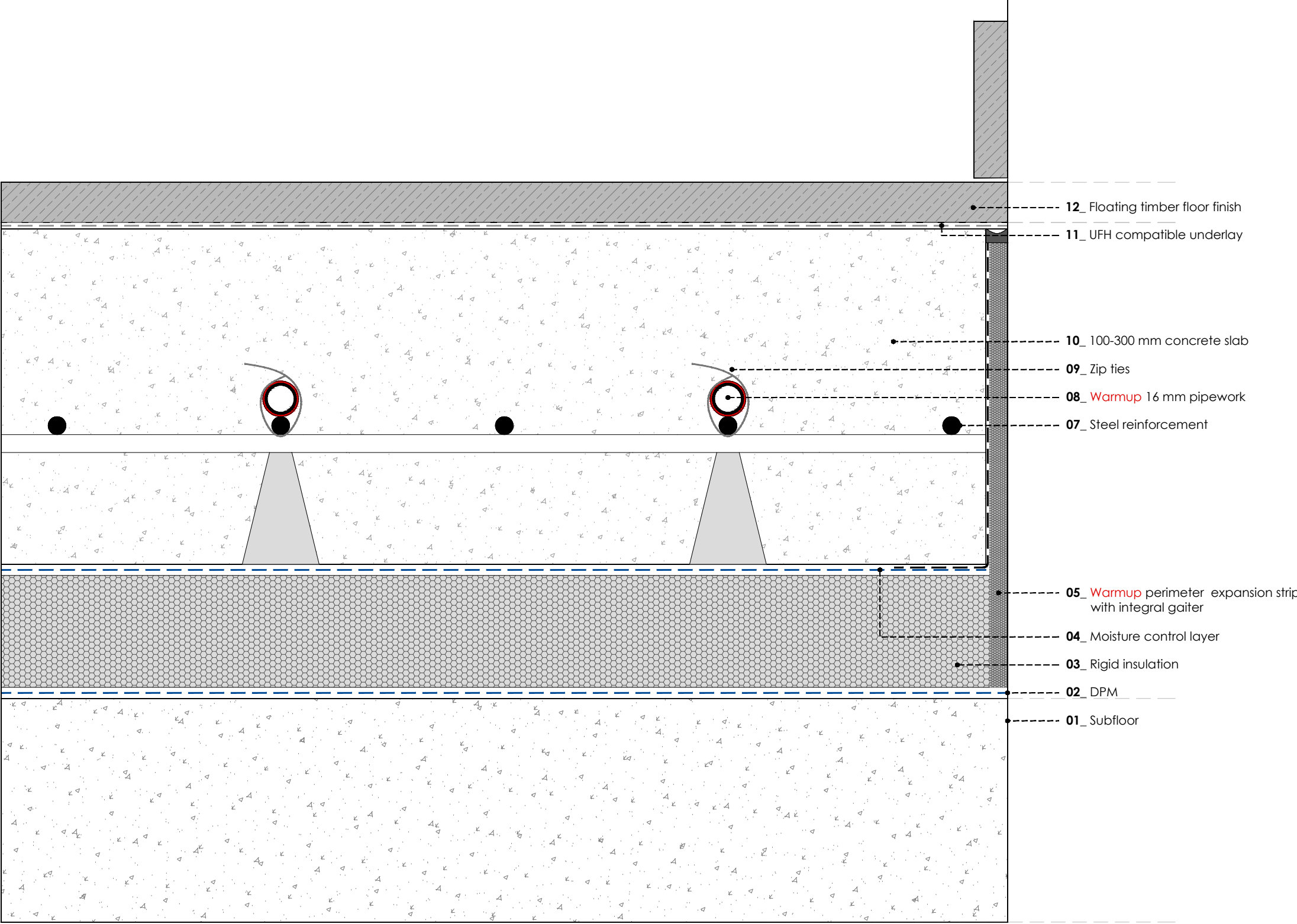
WARMUP FORTE GRID SYSTEM. Wood / Laminate floor - floating
