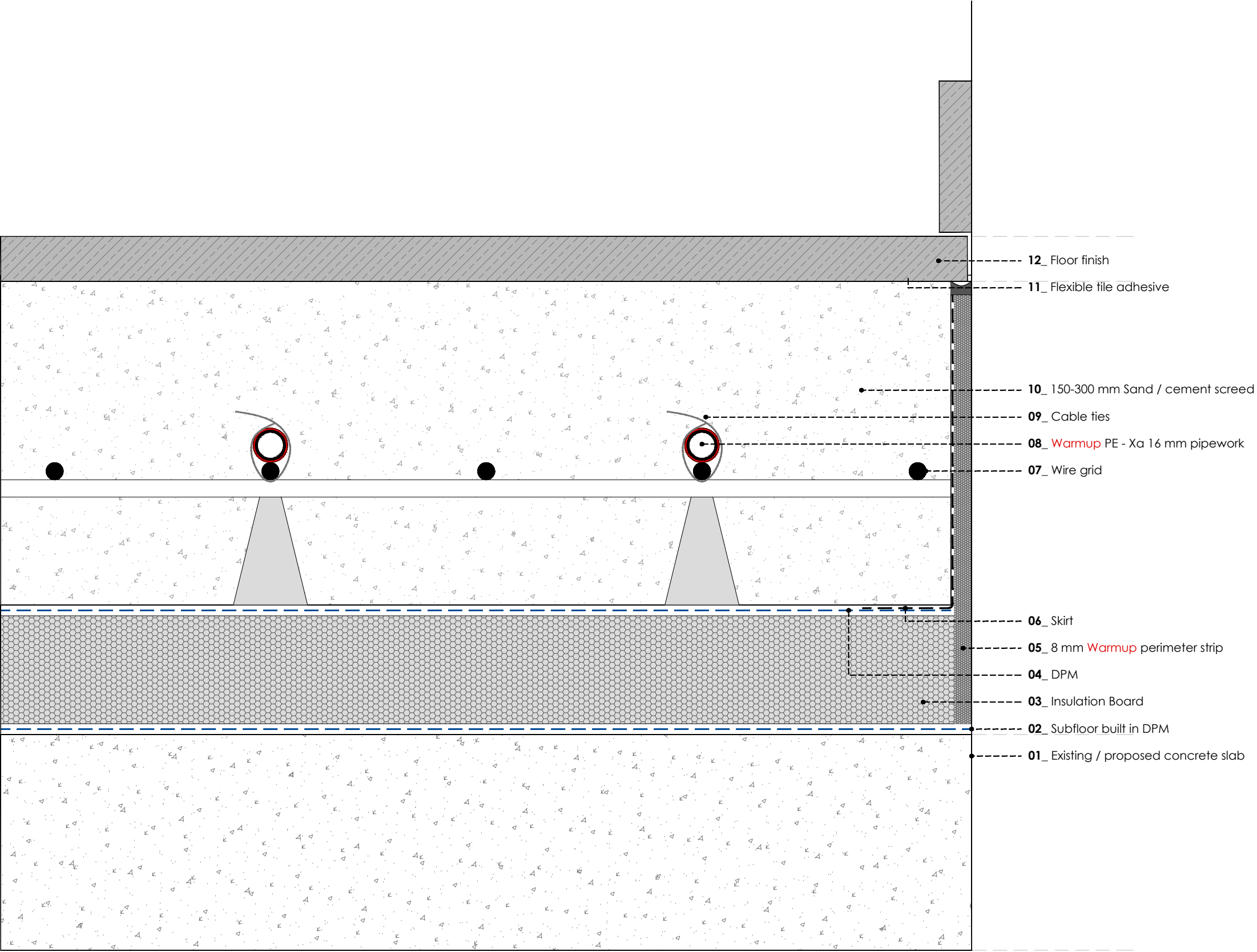
WARMUP FORTE GRID SYSTEM. Generic template
