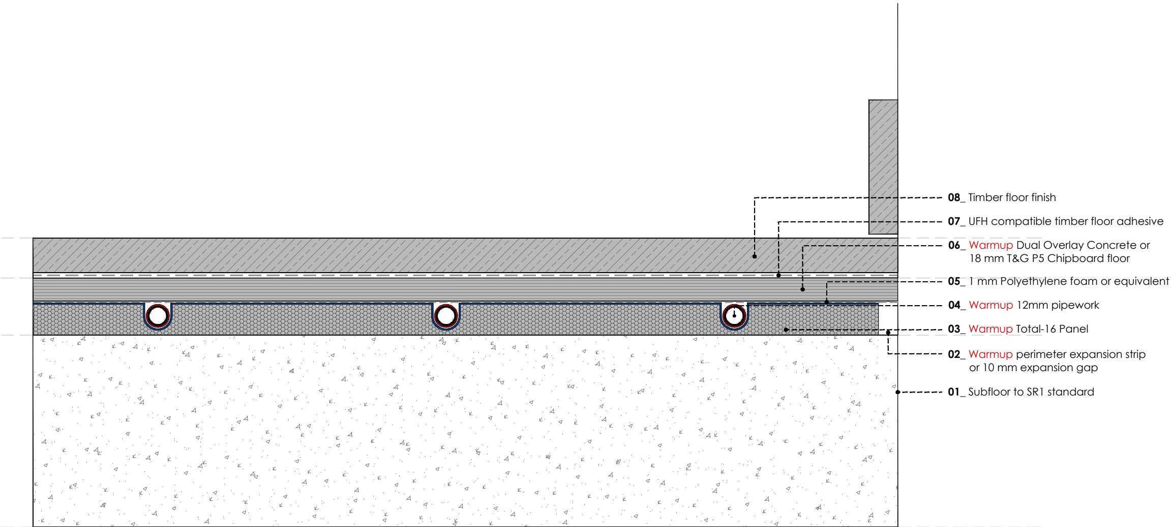
WARMUP TOTAL16. Concrete subfloor. Wood / Laminate floor - glued
