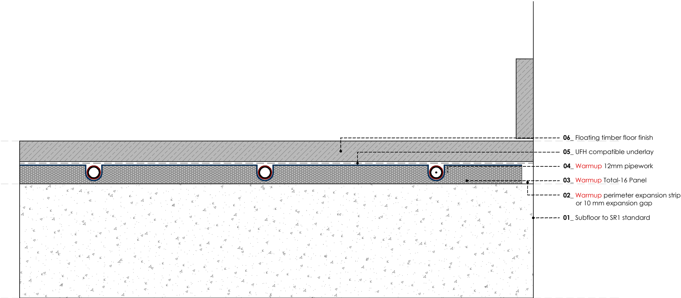
WARMUP TOTAL16. Concrete subfloor. 14-25 mm Wood / Laminate floor - floating
