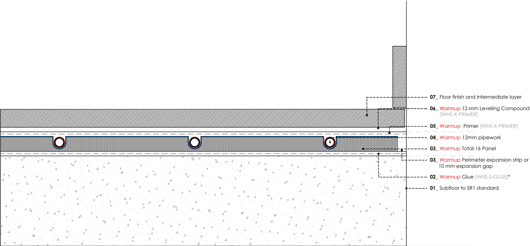
WARMUP TOTAL16. Concrete subfloor. Generic template
