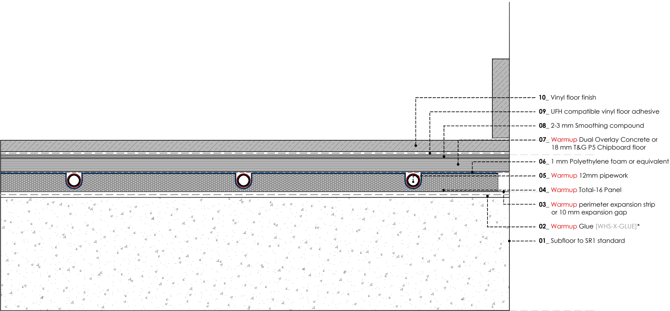
WARMUP TOTAL16. Concrete subfloor. Vinyl floor - floating
