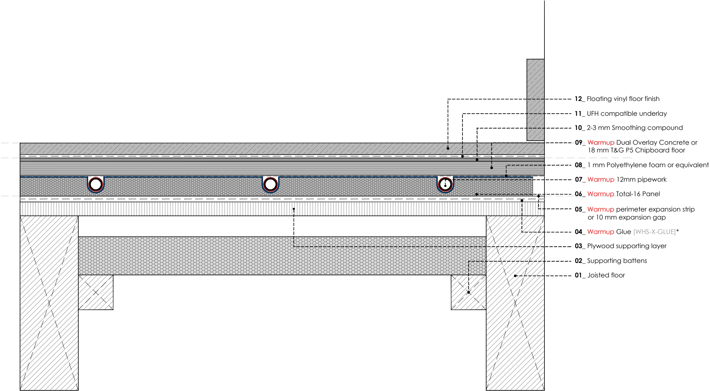
WARMUP TOTAL16. Timber subfloor. Vinyl floor - floating
