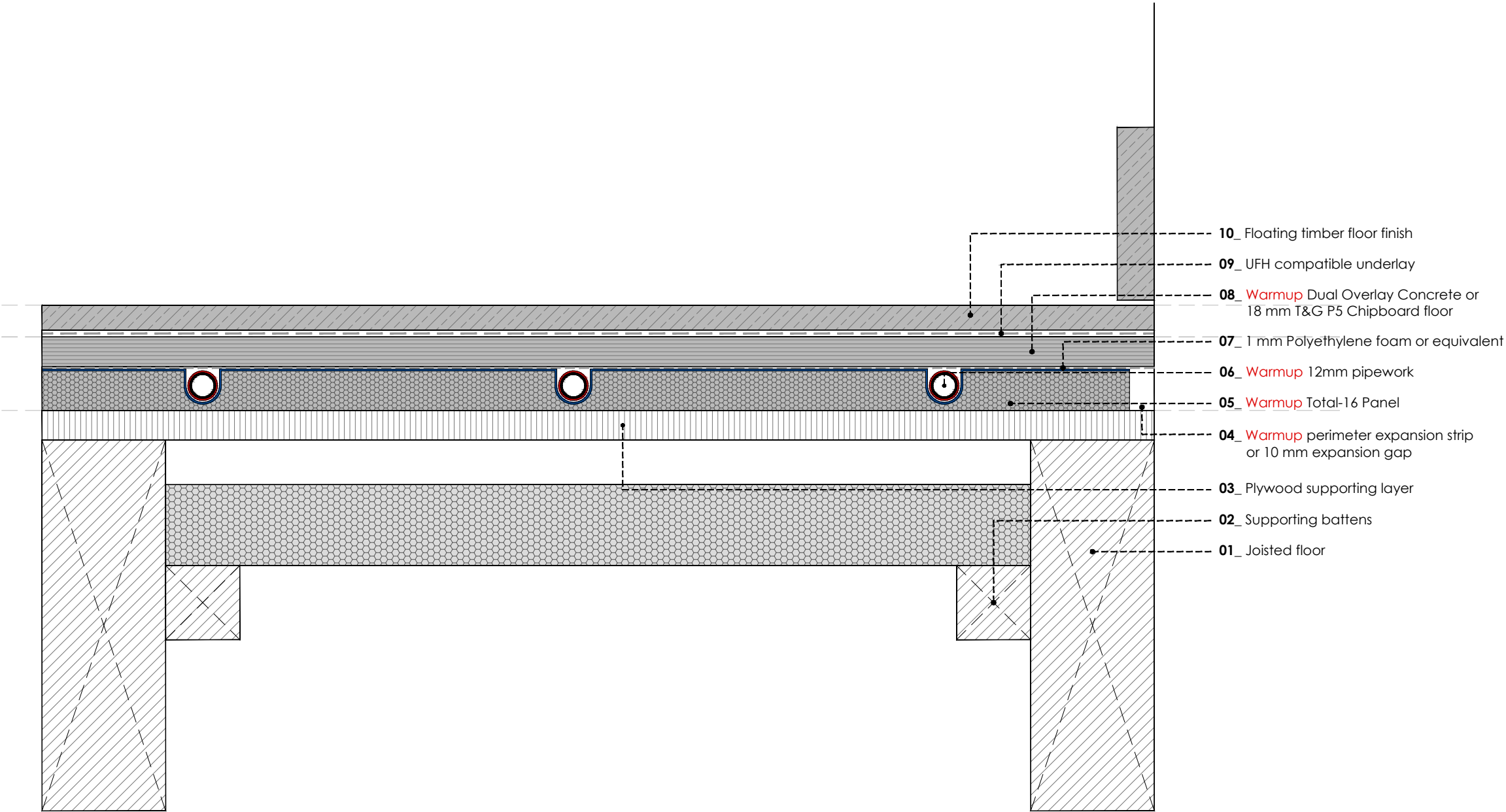
WARMUP TOTAL16. Timber subfloor. <14 mm Wood / Laminate floor - floating
