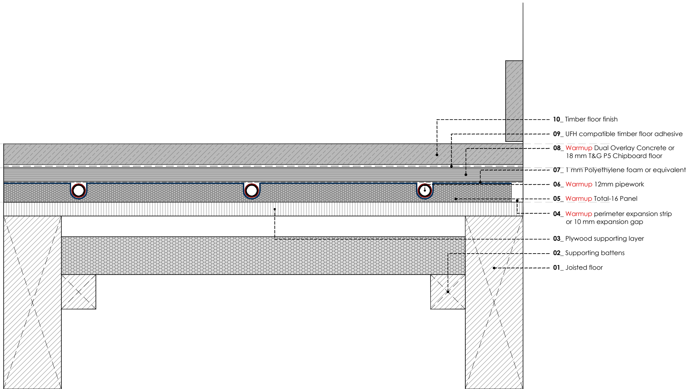
WARMUP TOTAL16. Timber subfloor. Wood / Laminate floor - glued
