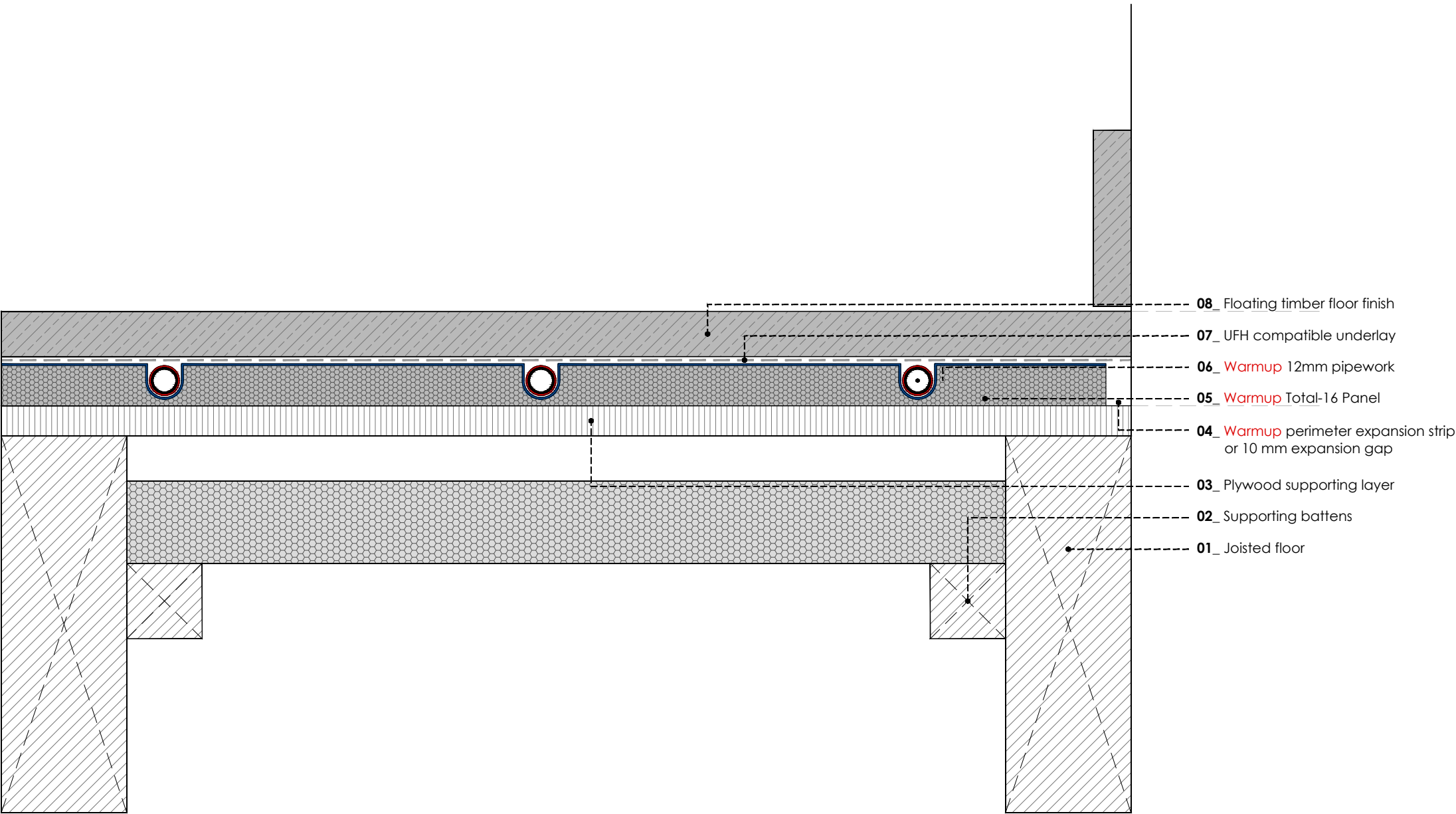
WARMUP TOTAL16. Timber subfloor. 14-25 mm Wood / Laminate floor - floating
