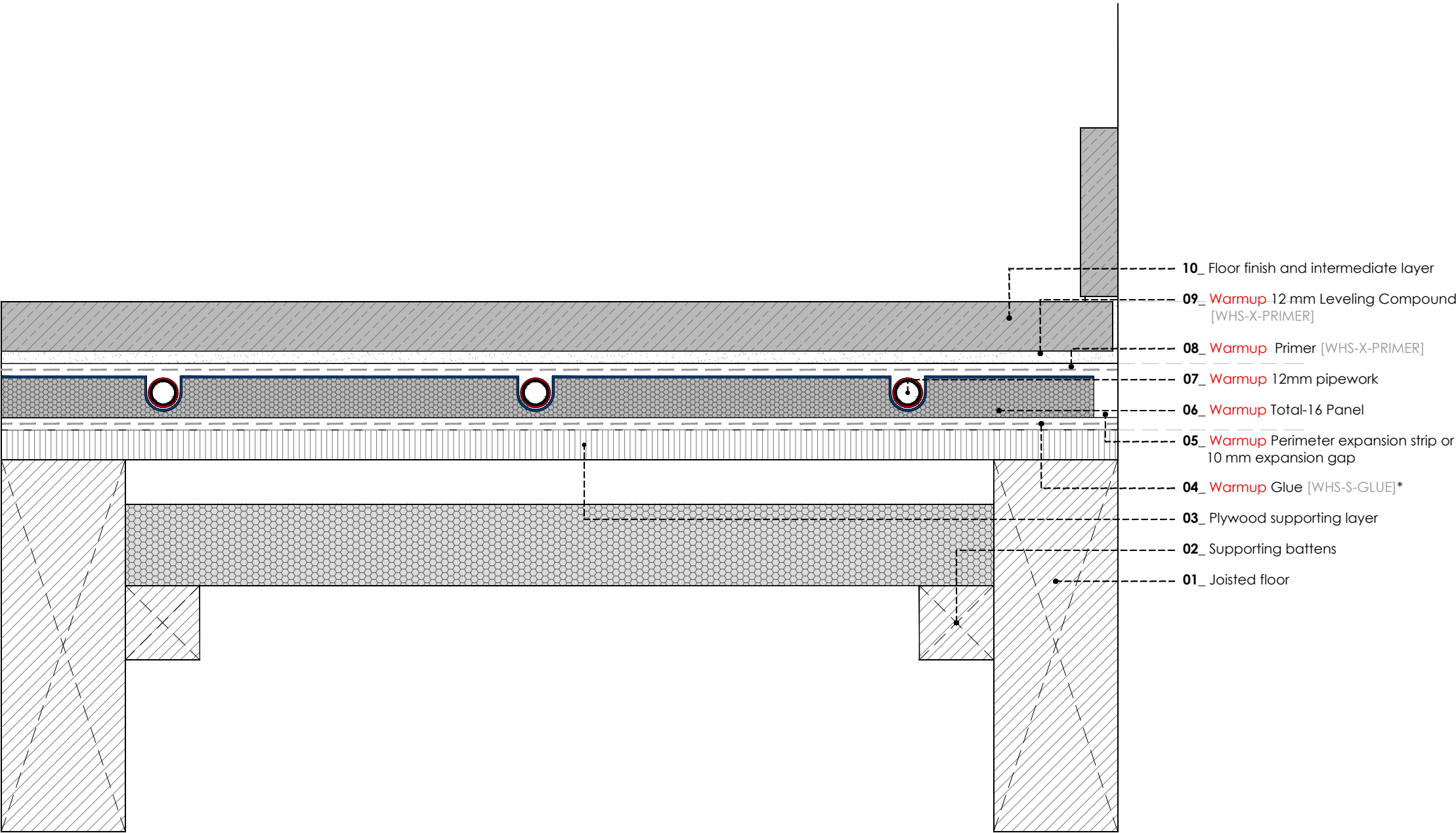
WARMUP TOTAL16. Timber subfloor. Generic template
