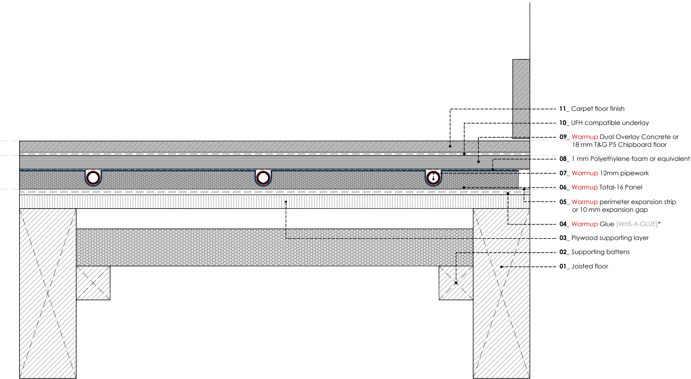
WARMUP TOTAL16. Timber subfloor. Carpet floor
