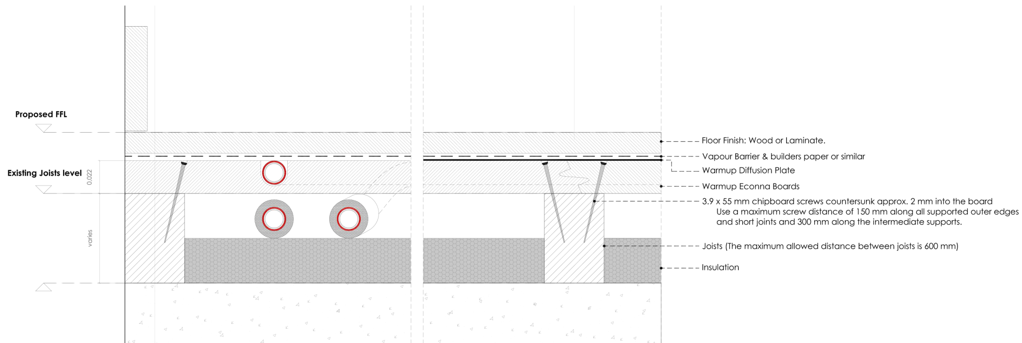
WOOD AN LAMINATE _Warmup Econnia Joisted Floor System
