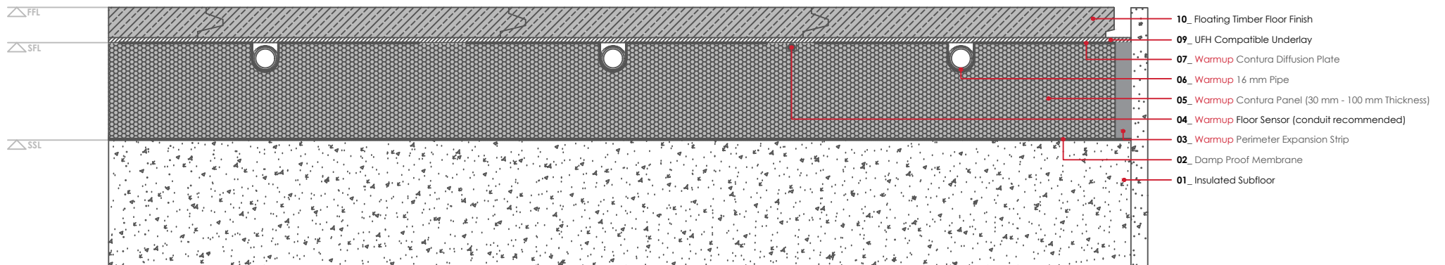
WARMUP CONTURA SYSTEM. Floating timber floor finish
