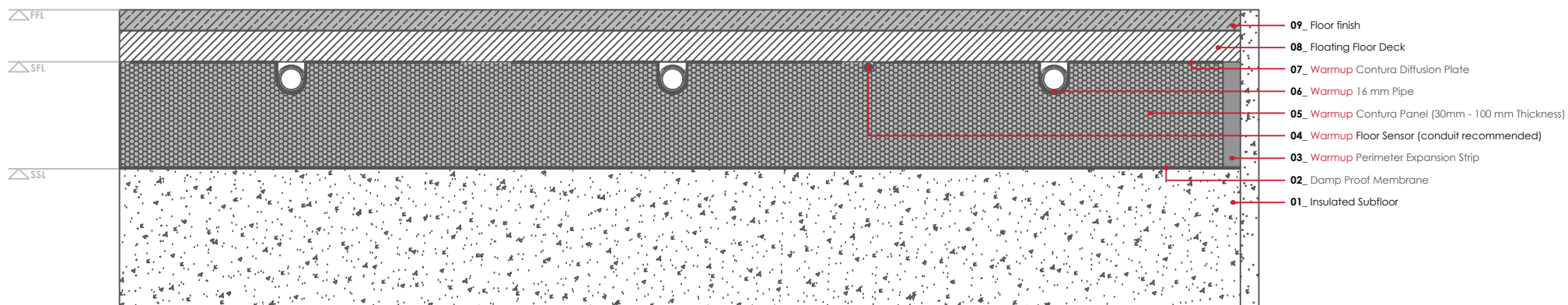
WARMUP CONTURA SYSTEM. Standard Detail
