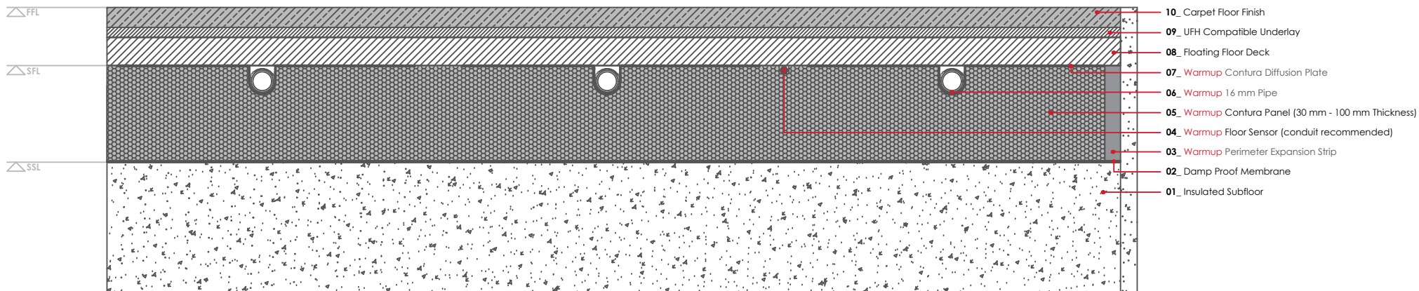
WARMUP CONTURA SYSTEM. Carpet floor finish
