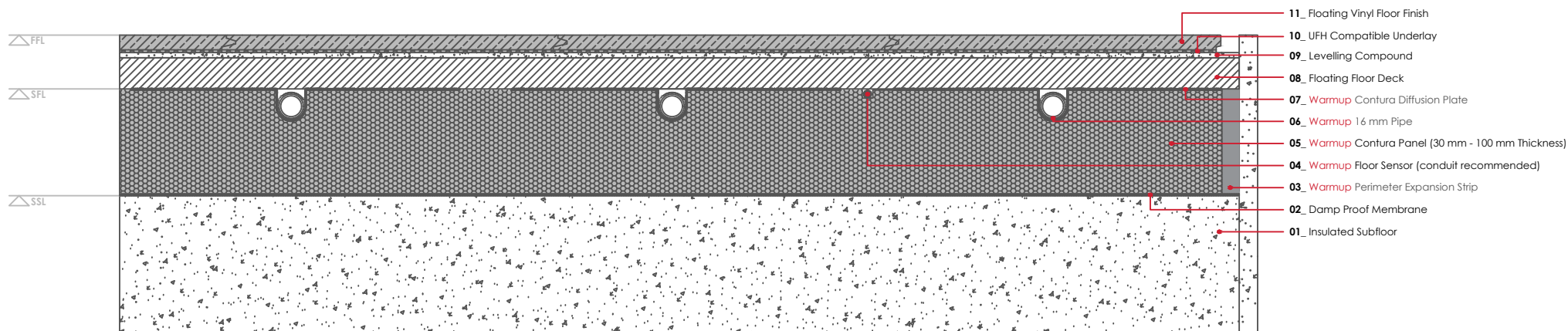
WARMUP CONTURA SYSTEM. Vinyl floor finish - floating
