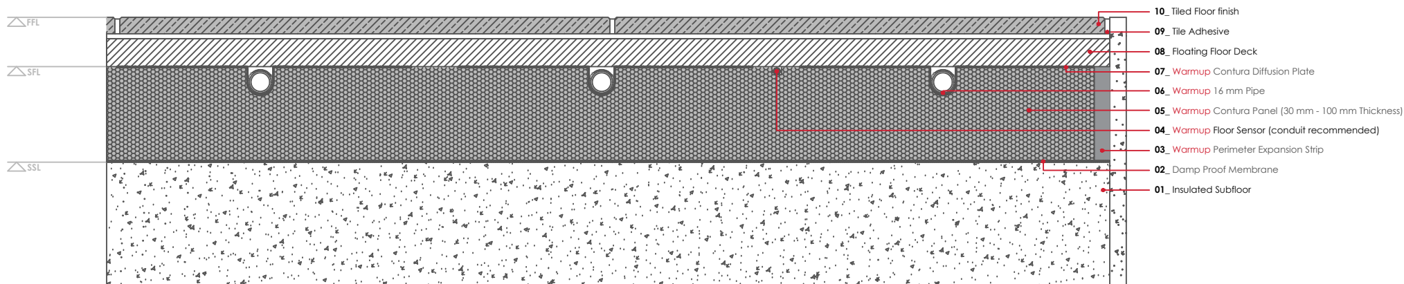
WARMUP CONTURA SYSTEM. Tiled floor finish
