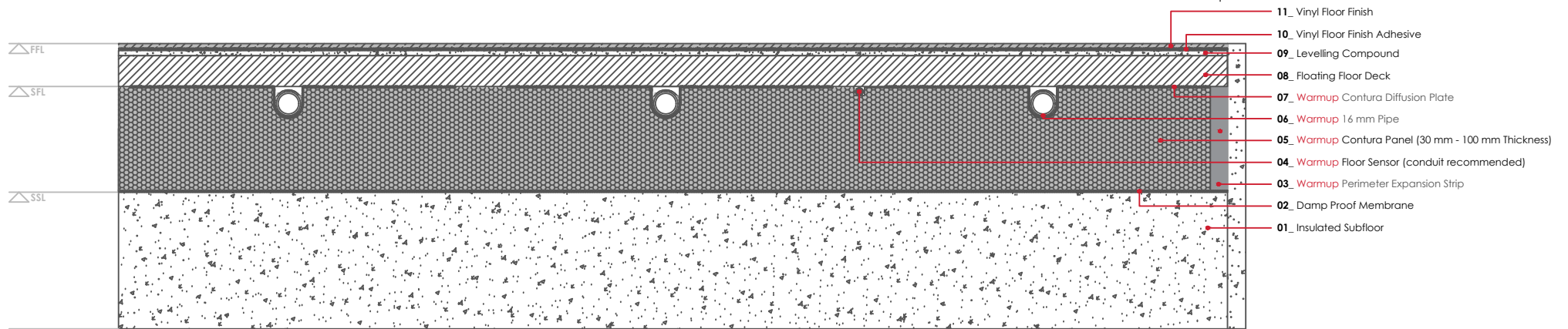
WARMUP CONTURA SYSTEM. Vinyl floor finish - glued
