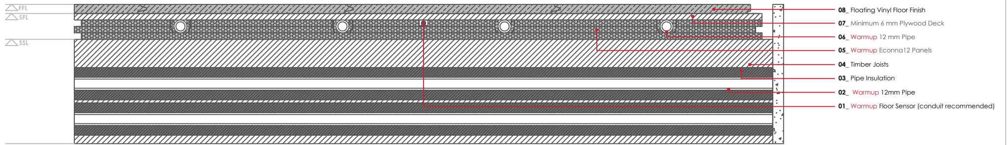
WARMUP Econna12 SYSTEM. Vinyl Floor Finish - Floating
