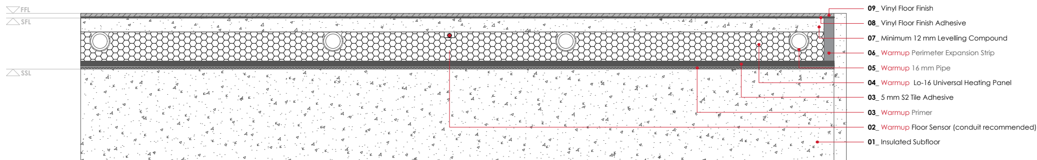
WARMUP Lo-16 SYSTEM. Vinyl floor finish - glued
