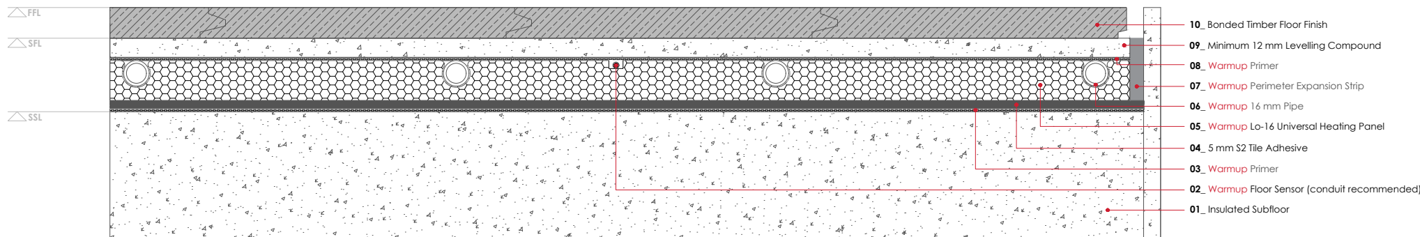
WARMUP Lo-16 Bonded timber floor finish
