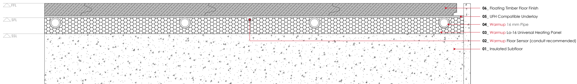
WARMUP Lo-16 Floating timber floor finish
