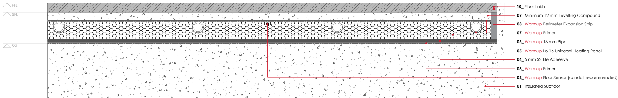
WARMUP Lo-16 SYSTEM. Standard Detail
