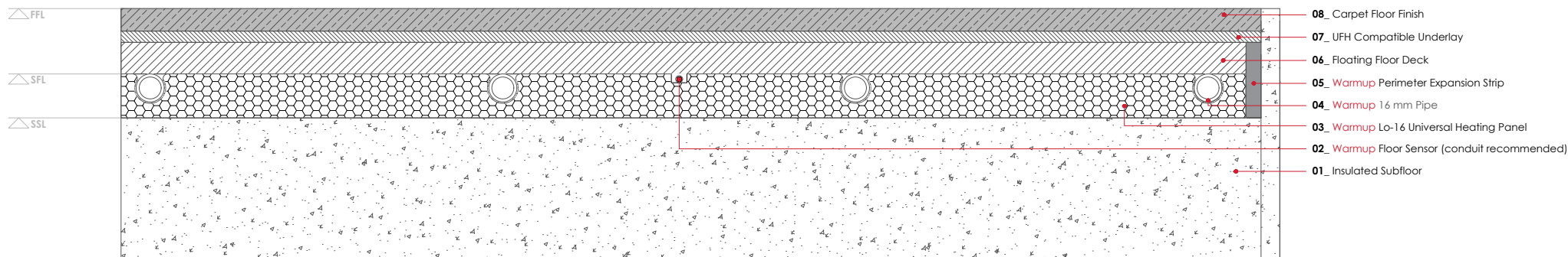
WARMUP Lo-16 SYSTEM. Carpet floor finish
