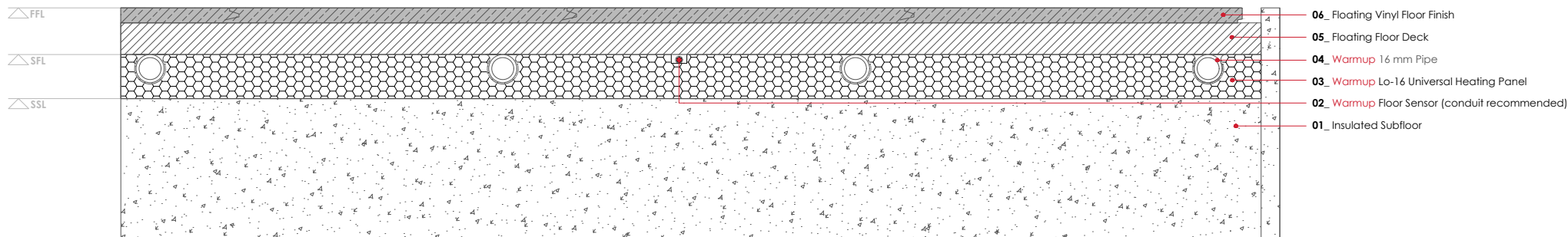
WARMUP Lo-16 SYSTEM. Vinyl floor finish - floating
