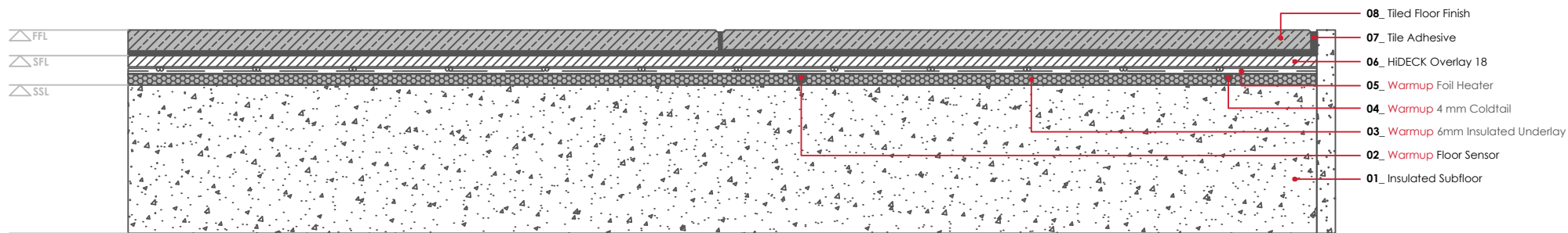
WARMUP FOIL HEATER SYSTEM Tiled floor finish
