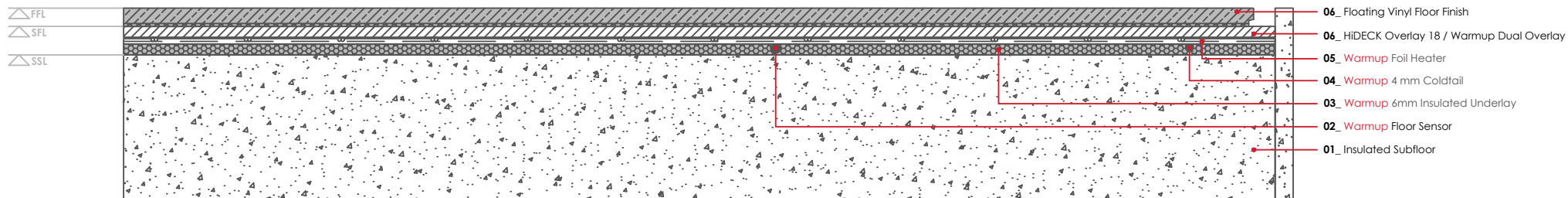
WARMUP FOIL HEATER SYSTEM. Vinyl floor finish - floating
