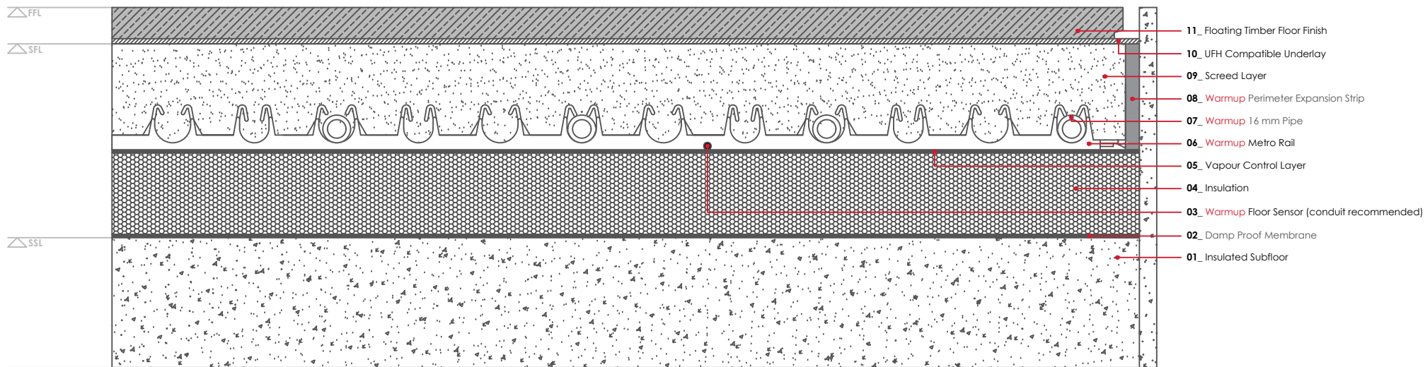
WARMUP METRO Floating timber floor finish
