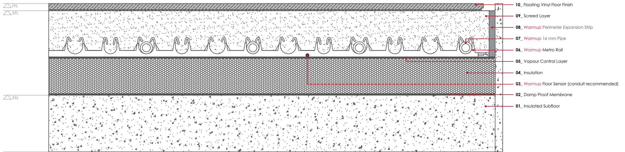
WARMUP METRO SYSTEM. Vinyl floor finish - floating
