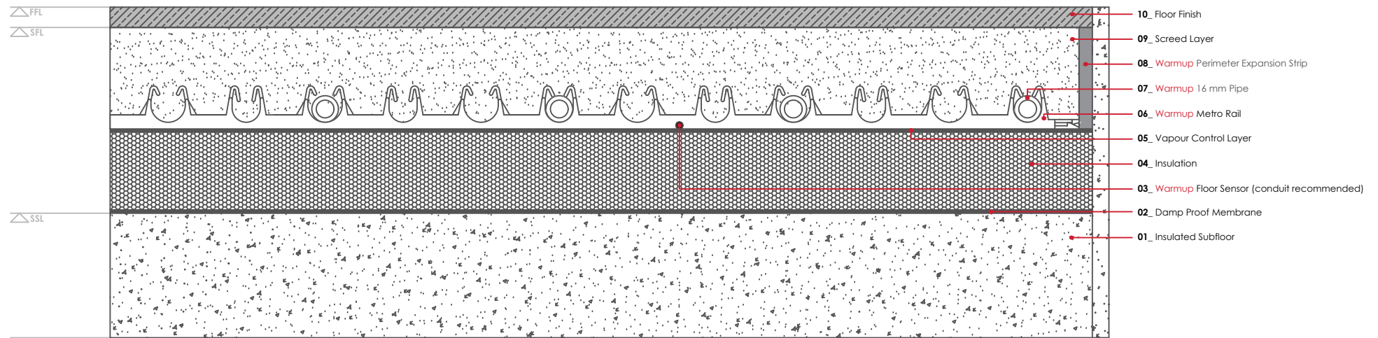
WARMUP METRO SYSTEM. Standard Detail
