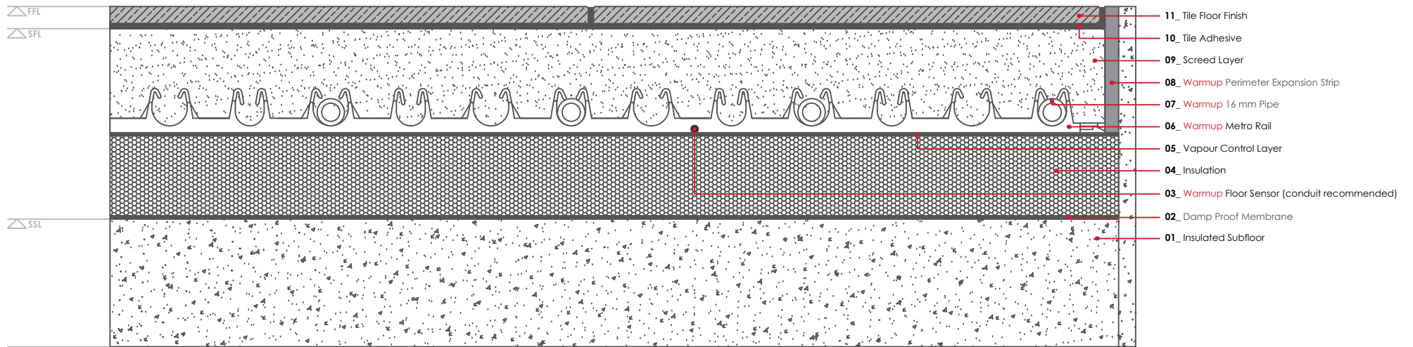
WARMUP METRO SYSTEM. Tiled floor finish
