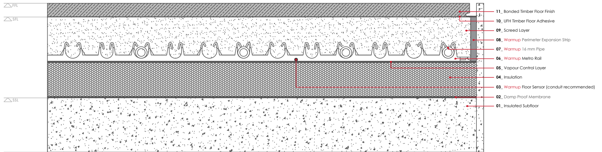
WARMUP METRO Bonded timber floor finish
