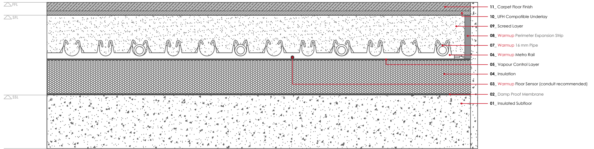
WARMUP METRO SYSTEM. Carpet floor finish
