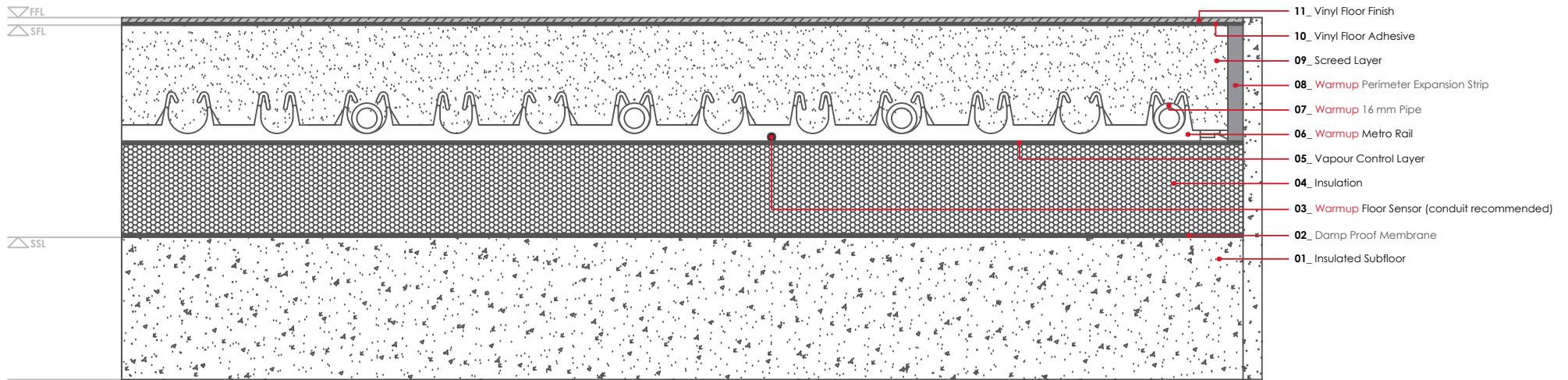
WARMUP METRO SYSTEM. Vinyl floor finish - glued
