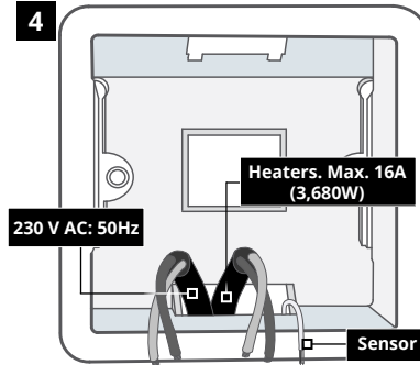
Floor Sensor
